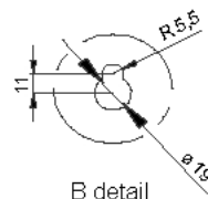
B detail
