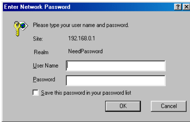
Figure 35: Password Dialog
