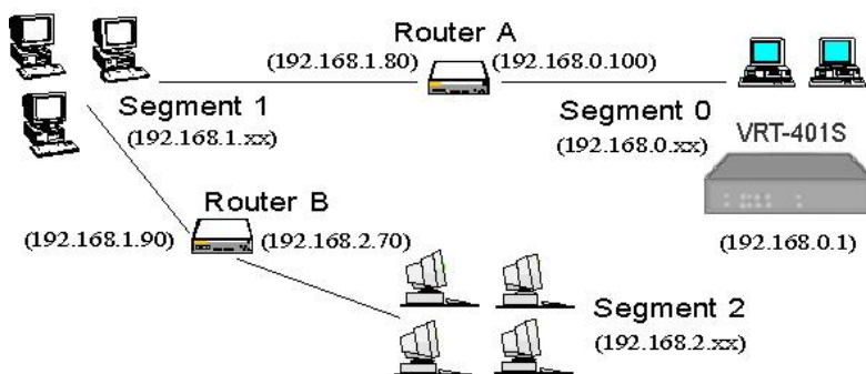
Figure 96: Routing Example
