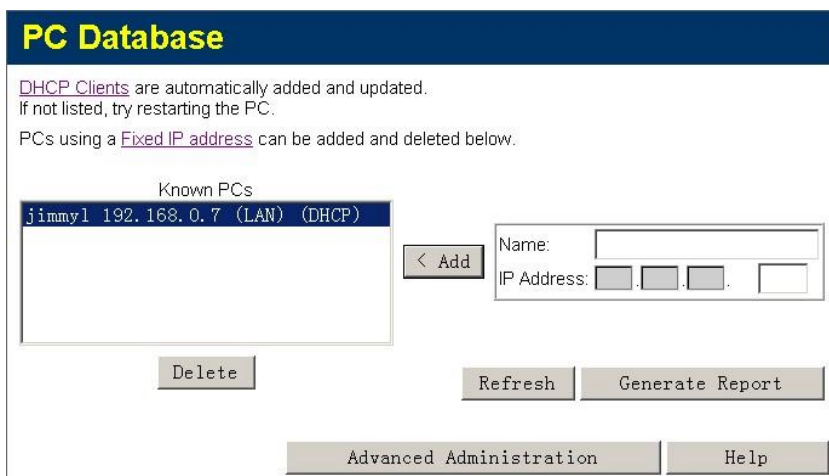
Figure 92: PC Database
