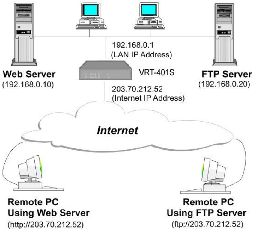
Figure 31: Virtual Servers
