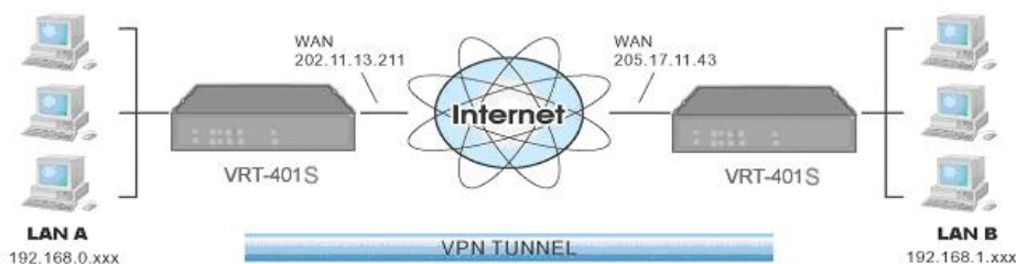
Figure 54: Connecting 2 VRT-401Ss
