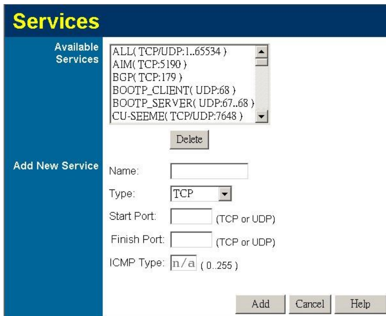
Figure 43: Services Screen
