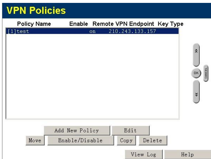
Figure 47: VPN Policies
