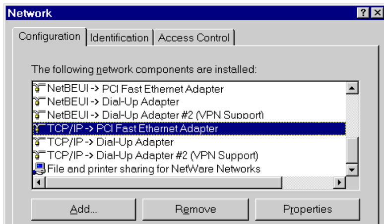
Figure 9: Network Configuration
