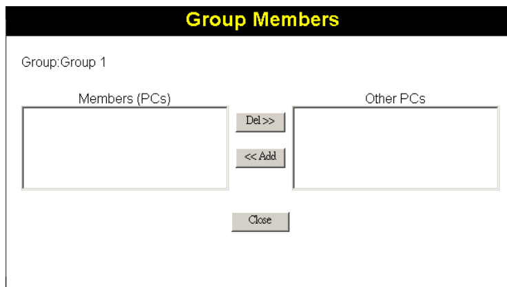
Figure 37: Group Members
