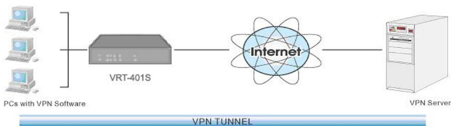
Figure 44: VPN Pass-through
