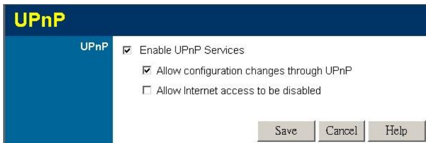
Figure 98: UPNP Screen
