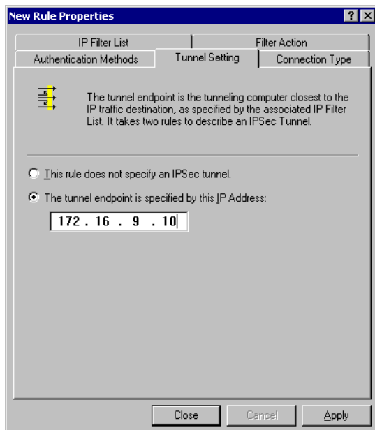
Figure 74: Tunnel Setting
