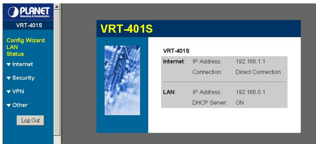
Figure 6: Home Screen
