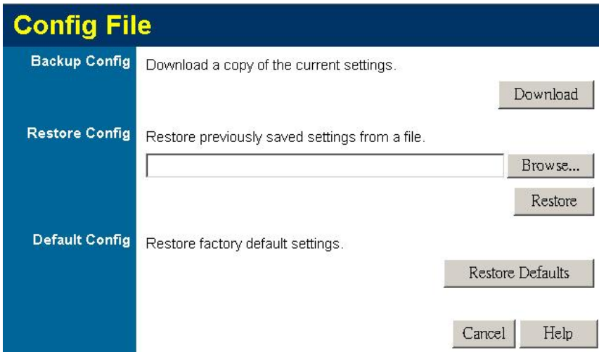
Figure 91: Config Screen
