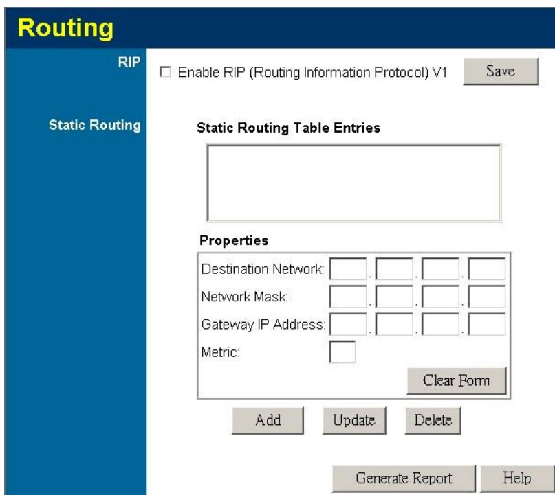
Figure 95: Routing Screen
