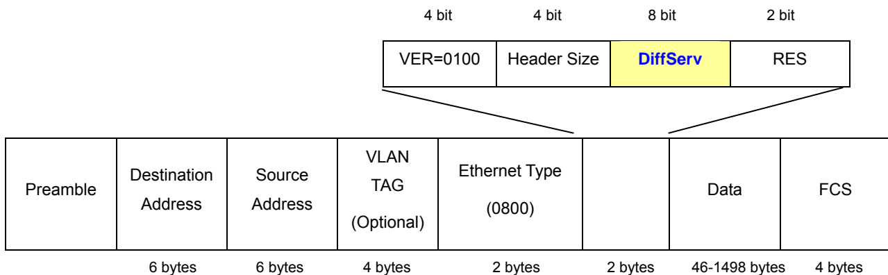
Figure 4-9-4: IPv4 frame format
