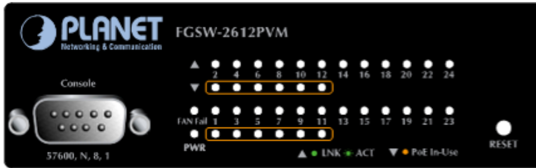
Figure 2-1-9: FGSW-2612PVM LED panel
