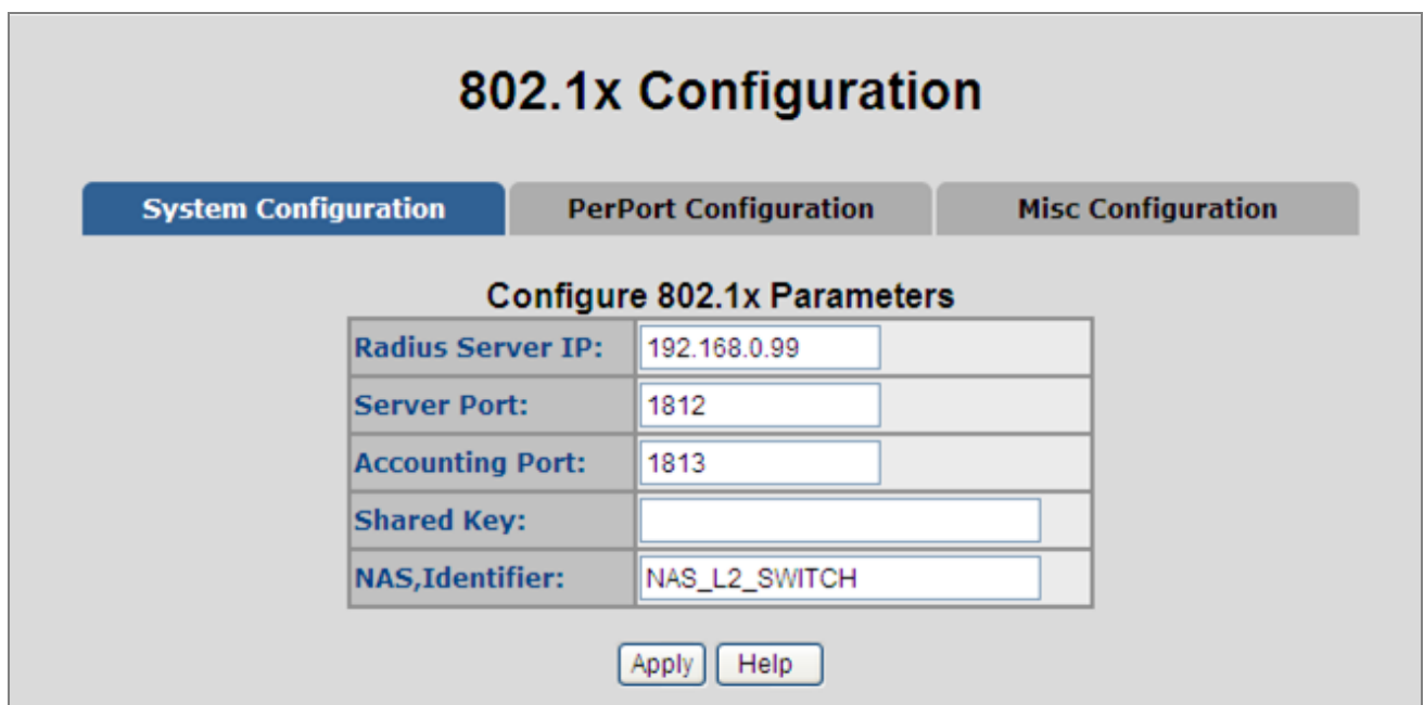
Figure 4-13-4: 802.1x System Configuration interface
