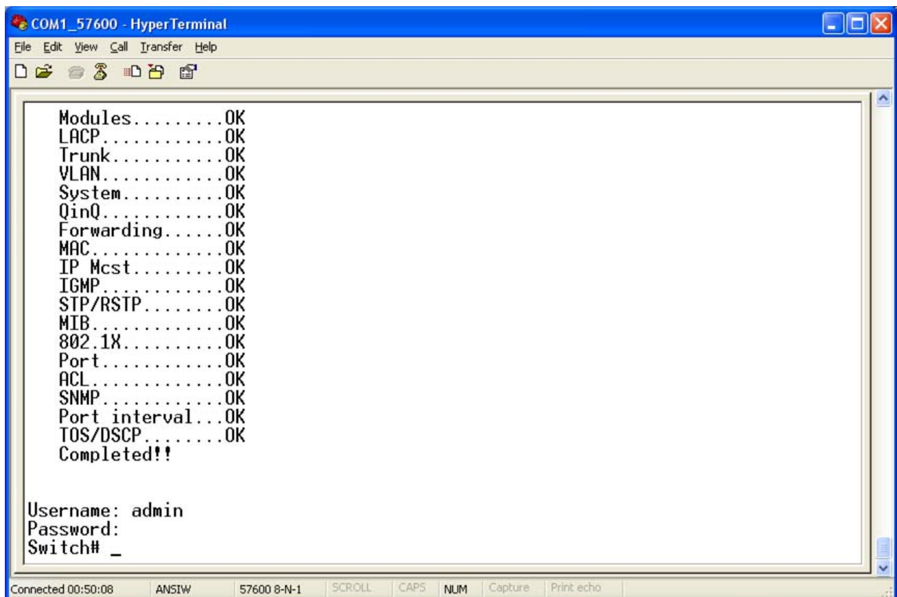
Figure 5-1-1: Console Login screen
