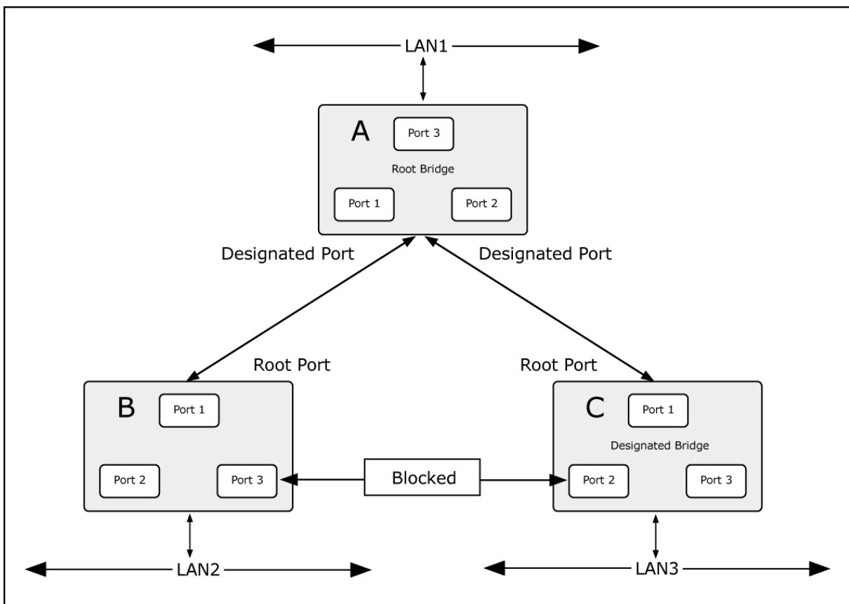
Figure 4-5-3: After Applying the STA Rules
