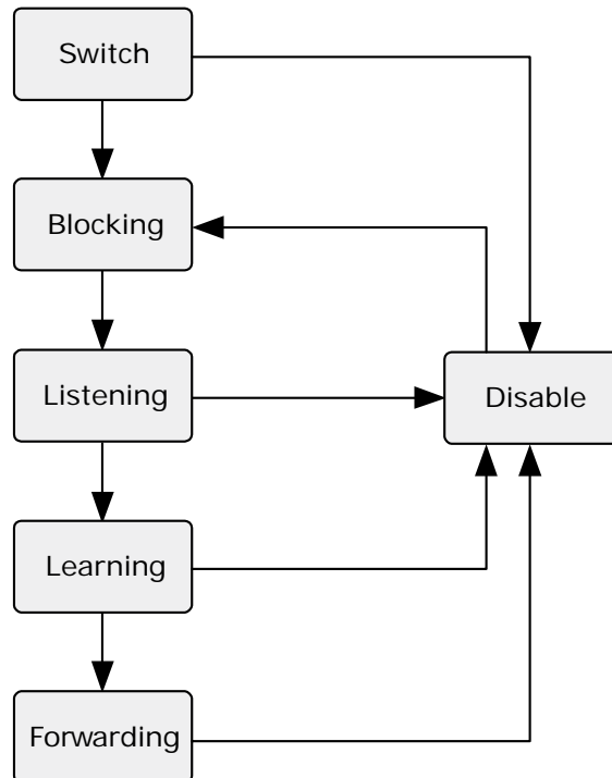
Figure 4-5-1: STP Port State Transitions
