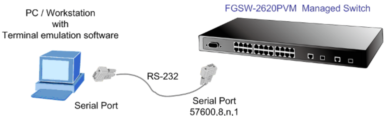
Figure 3-5-1: Console management
