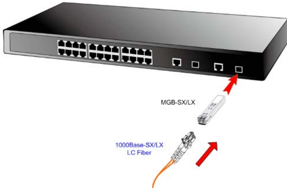
Figure 2-2-4: Plug-in the SFP transceiver
