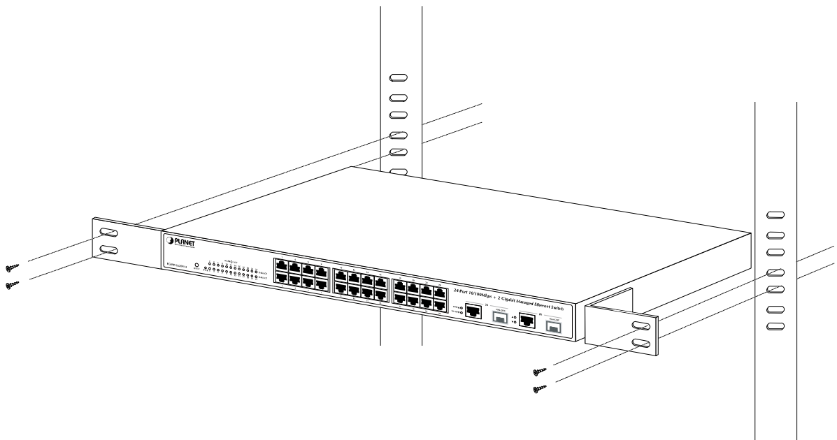
Figure 2-2-3: Mounting the Switch in a Rack
