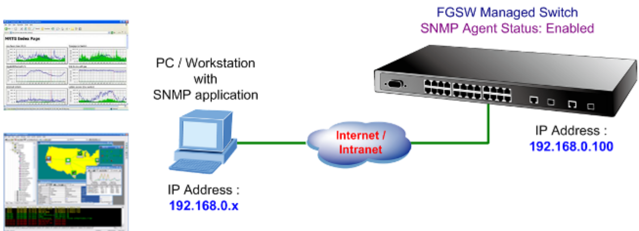
Figure 3-4-1: SNMP management
