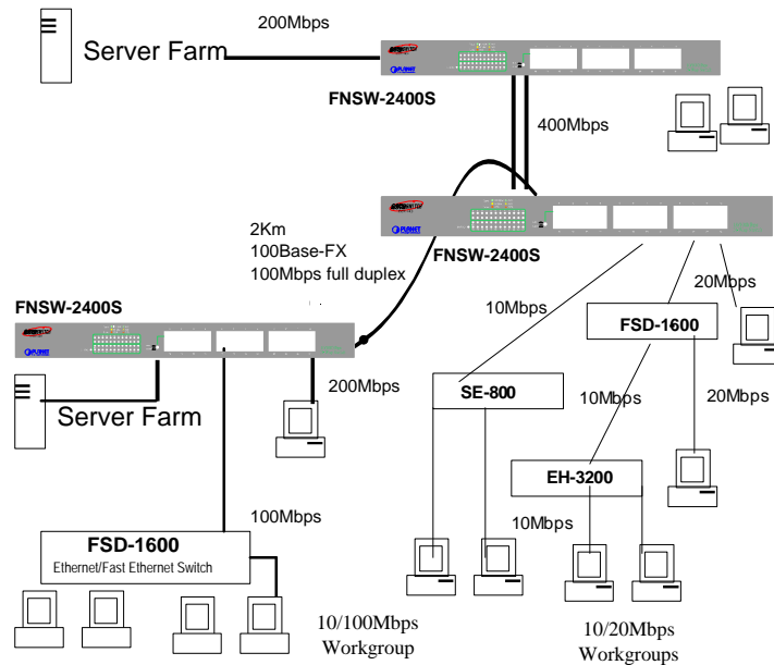
Figure 3: Sample Application for FNSW-2400S with Turnk
