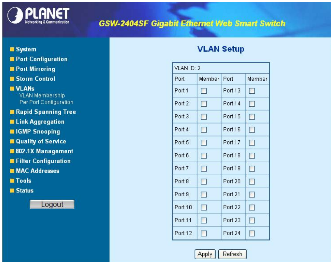
Figure 4-8 VLAN Member Setup screen
