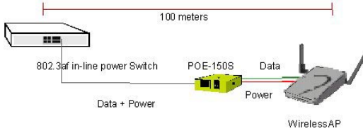
Figure 8: Connection to 802.3af in-line power switch
