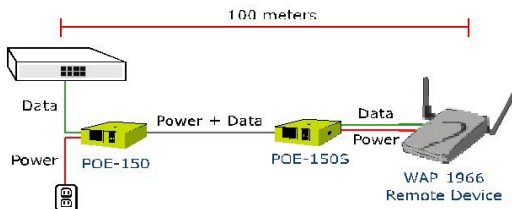
Figure 6: Connection architecture over POE-150/150S
