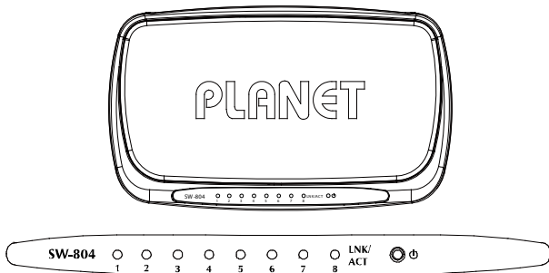
Figure 2-3 SW-804 front panel
