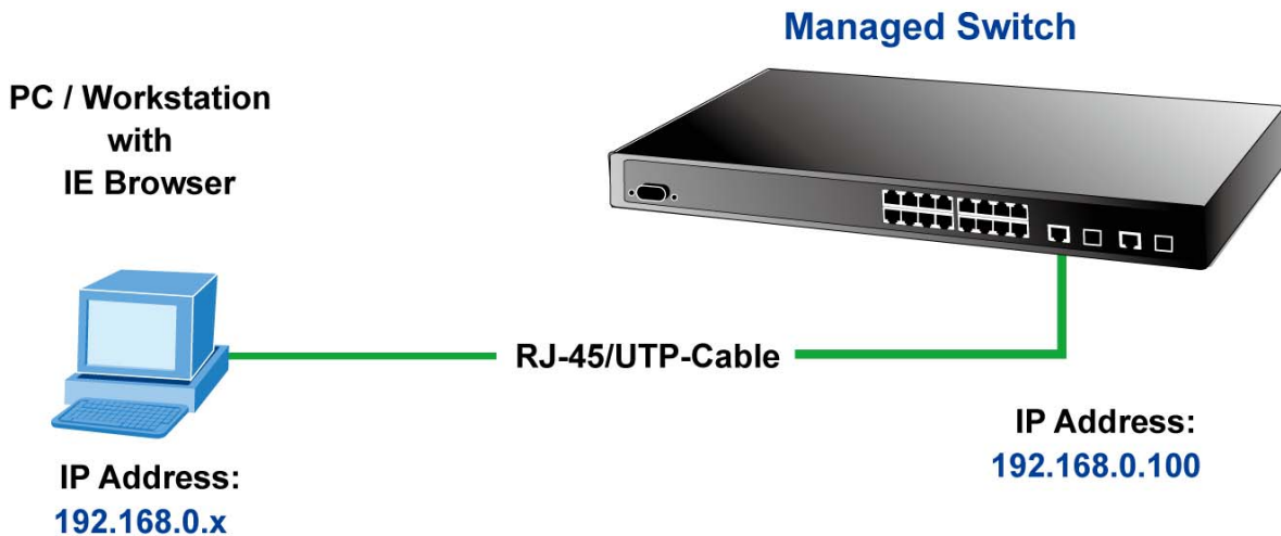
Figure 3-3-1 Web management
