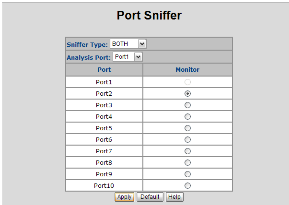
Figure 4-3-5: Port Sniffer interface
