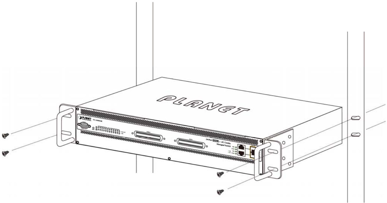
Figure 2-2-3: Mounting the VC-2400MR series in a Rack
