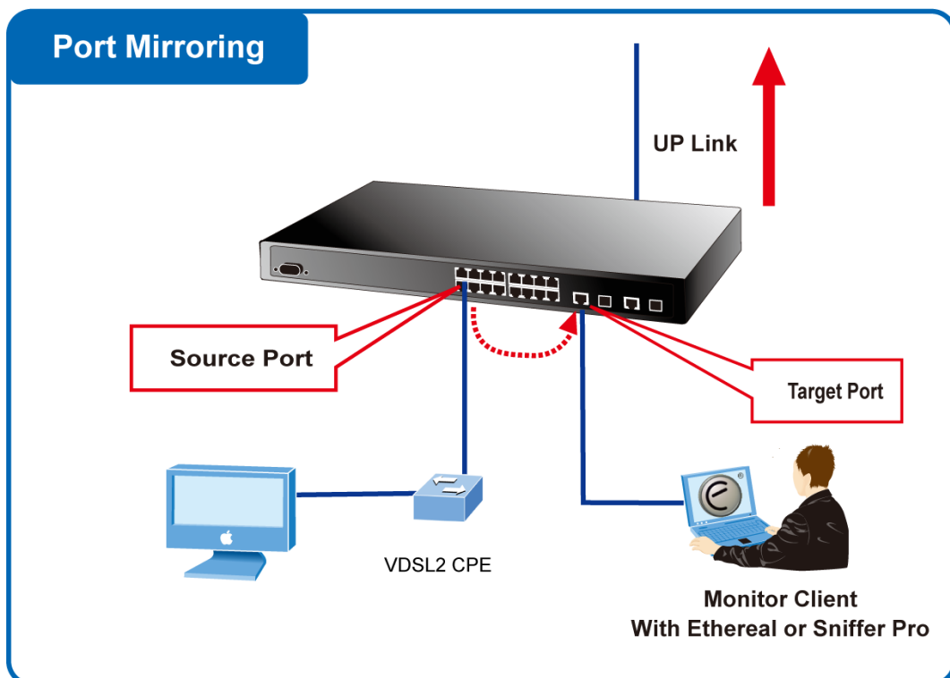
Figure 4-3-4: Port Mirror application
