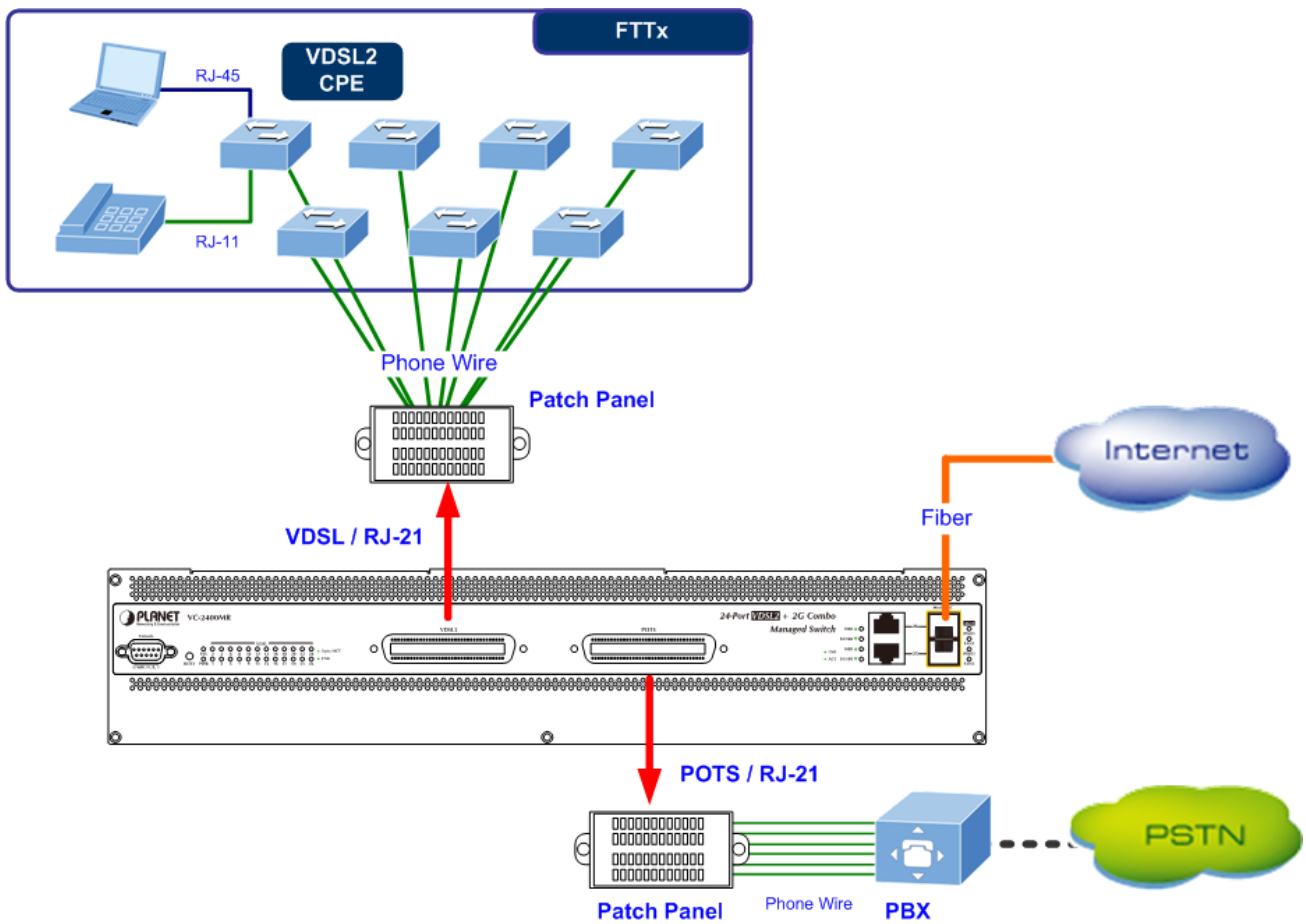
Figure 2-3-3: VC-2400MR Series VDSL2 connection
