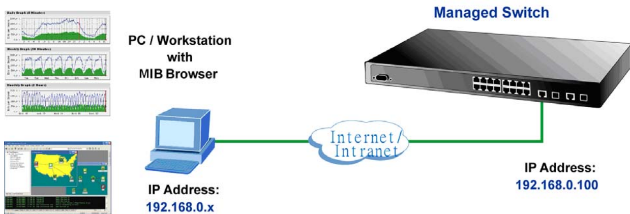
Figure 3-4-1 SNMP management
