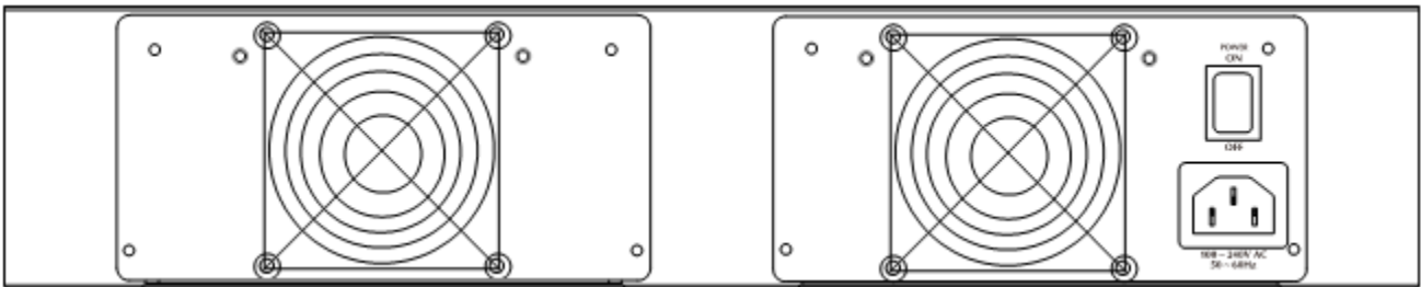
Figure 2-1-7: VC-2400MR rear panel with AC power module
