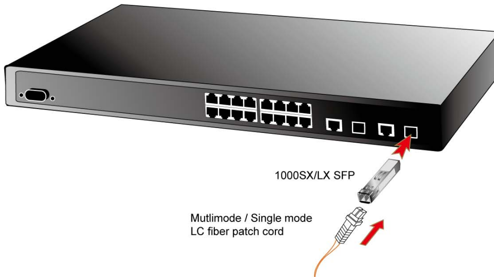
Figure 2-2-5: Plug-in the SFP transceiver
