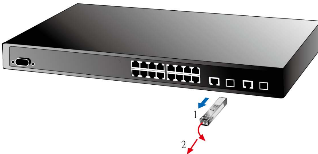
Figure 2-2-6: Pull out the SFP transceiver
