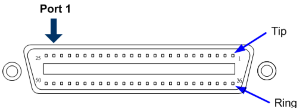
Figure 2-3-1 Pin out convention for the Telco RJ-21 connector of VC-2400MR series
