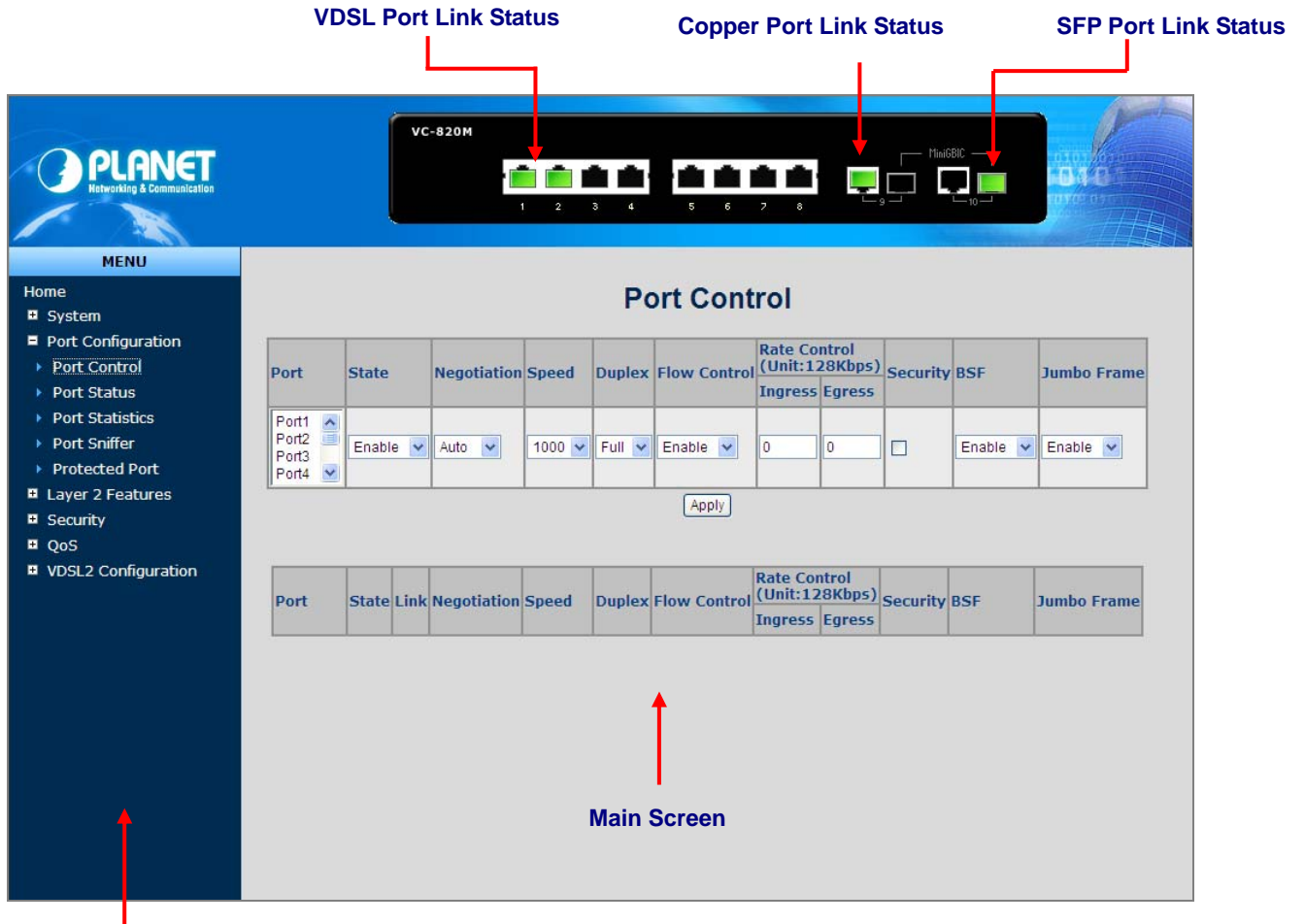
Figure 4-1-3: Main Page
