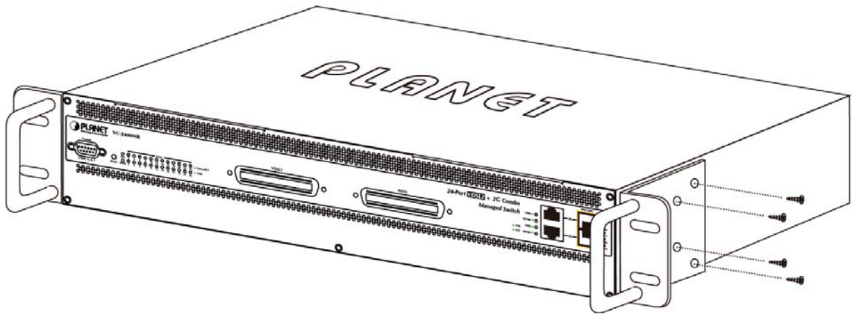
Figure 2-2-1 Attach brackets to VC-2400MR series
