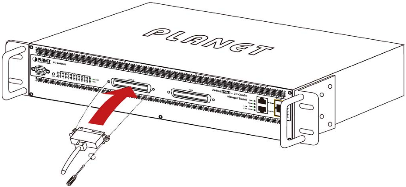
Figure 2-3-2 Telco RJ-21 connect to VC-2400MR series
