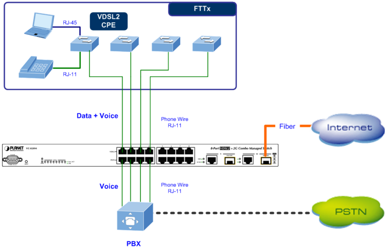
Figure 2-3-4: VC-820M VDSL2 connection
