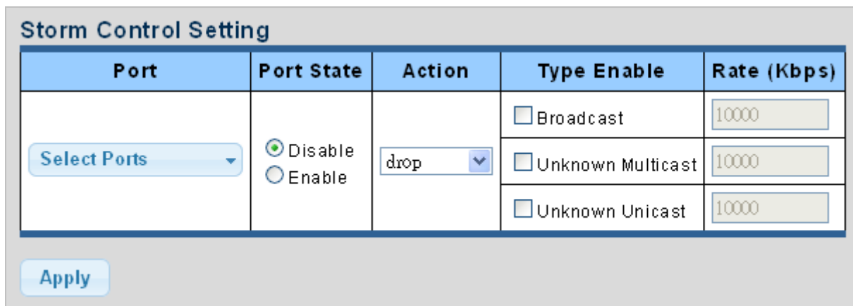
Figure 4-9-71 Storm Control Setting Page Screenshot
