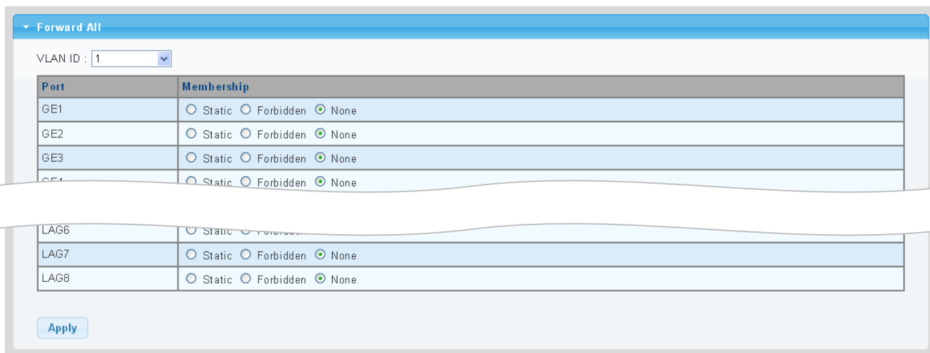
Figure 4-7-20 Forward All Setting Page Screenshot
