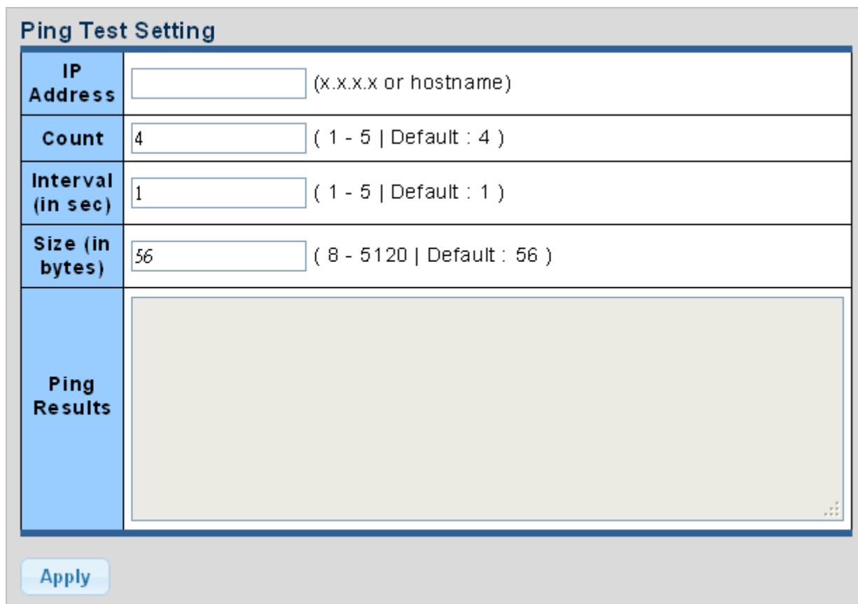
Figure 4-13-3 ICMP Ping Page Screenshot
