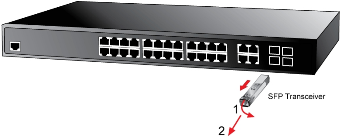
Figure 2-1-8 How to Pull Out the SFP Transceiver
