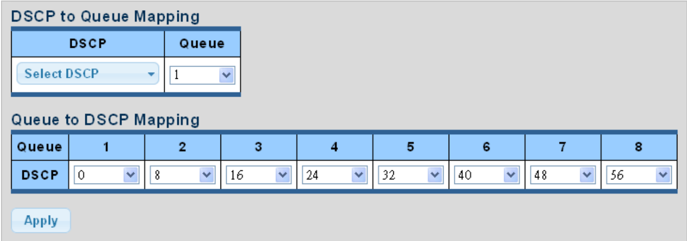
Figure 4-8-8 DSCP to Queue and Queue to DSCP Mapping Page Screenshot
