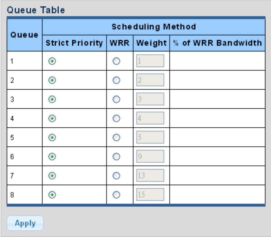
Figure 4-8-4 Queue Table Page Screenshot
