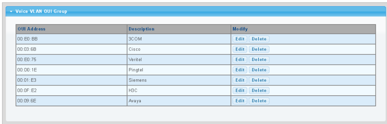
Figure 4-8-25 Voice VLAN OUI Group Page Screenshot
