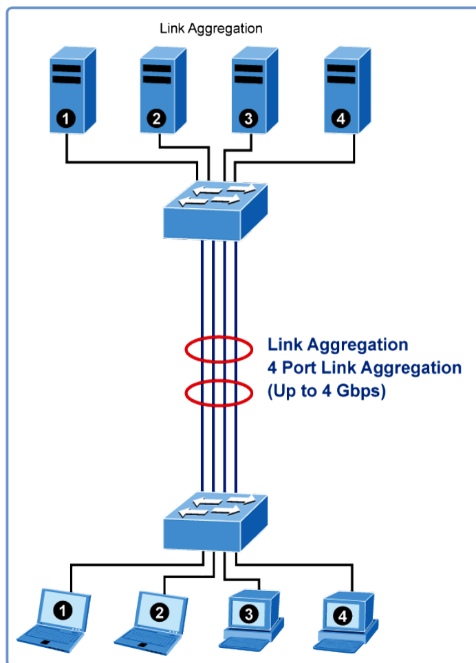
Figure 4-4-1 Link Aggregation
