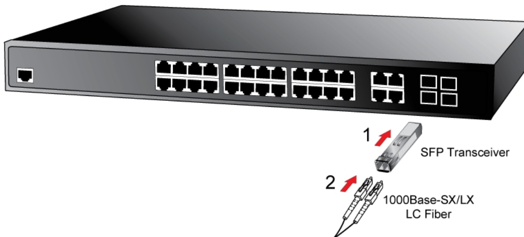
Figure 2-1-7 Plug in the SFP transceiver
