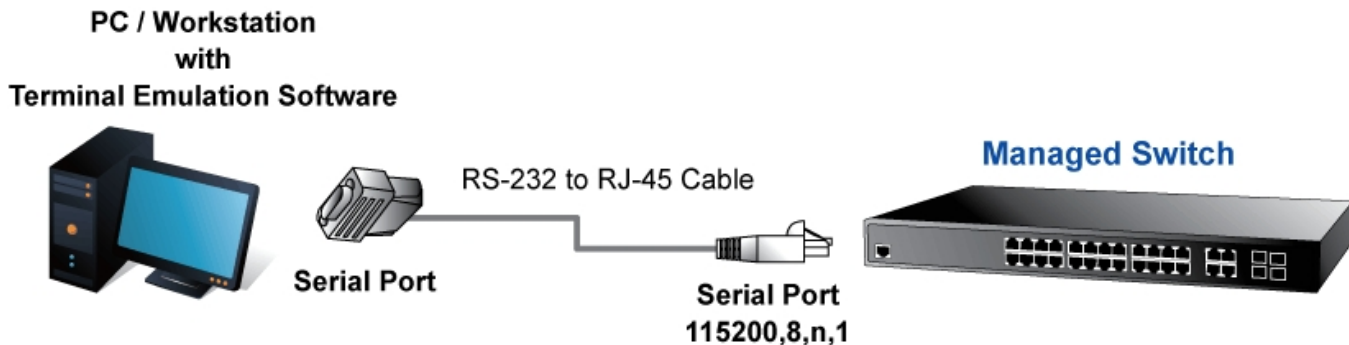
Figure 3-1-1: Console Management
