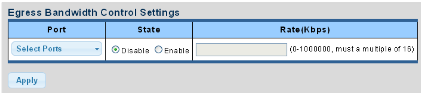
Figure 4-8-18 Egress Bandwidth Control Settings Page Screenshot
