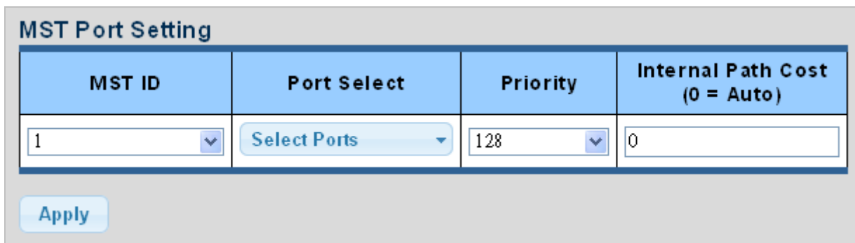
Figure 4-6-15 MST Port Configuration Page Screenshot
