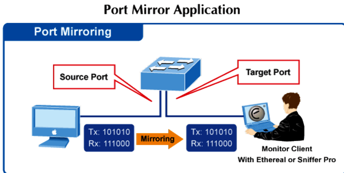
Figure 4-3-8 Port Mirror Application
