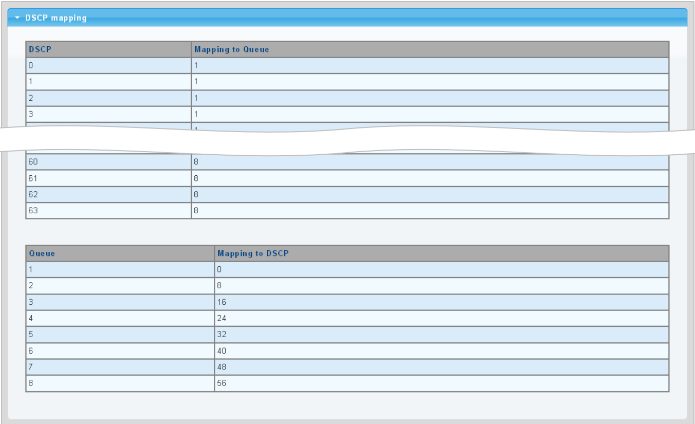
Figure 4-8-9 DSCP Mapping Page Screenshot
