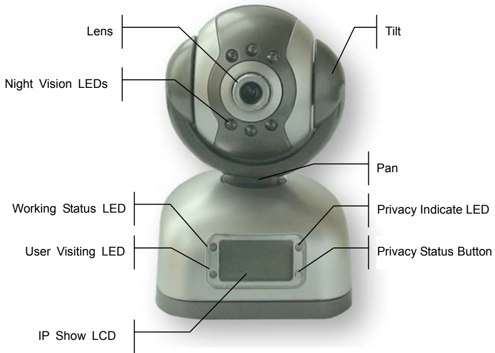
Figure 2 IP Camera Front View
