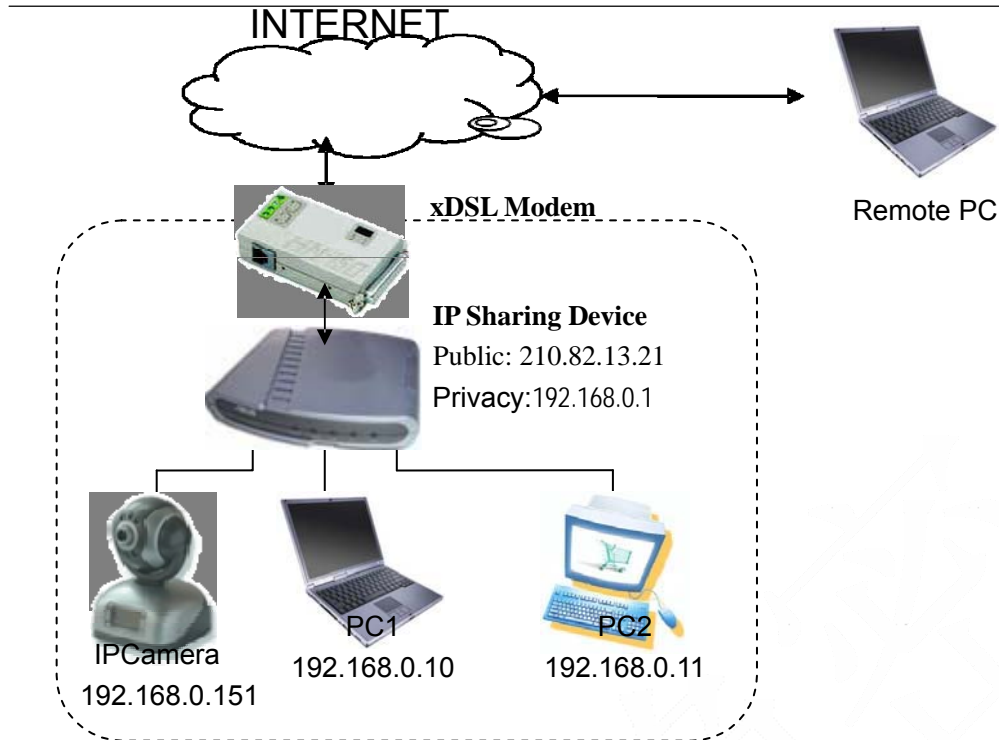
Figure 41 Typical Network Environment
