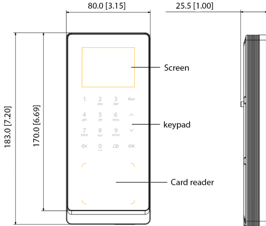
Figure 1-2 Dimensions (2) (mm[inch])
