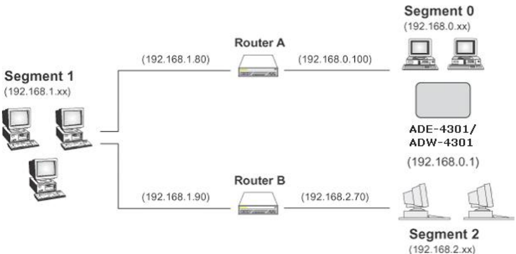
Figure 66: Routing Example
