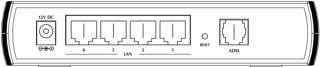
Figure 4: Rear Panel of ADE-4301
