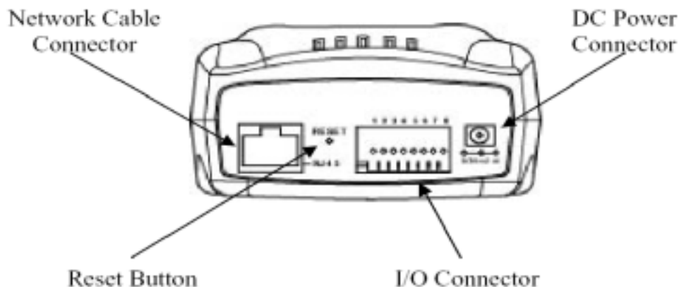
Figure 1-2: Rear panel of ICA-100
