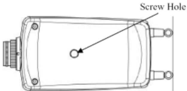
Figure 1-5 Bottom Panel
