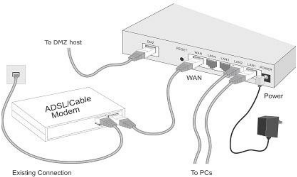
Figure 4: Installation Diagram
