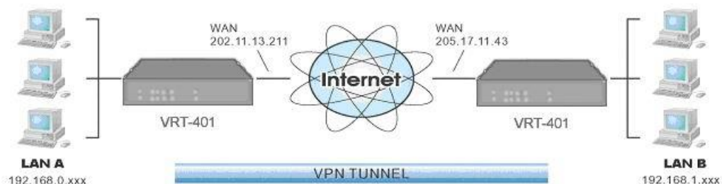
Figure 53: Connecting 2 VRT-401s
