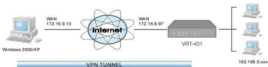
Figure 54: Windows 2000/XP Client to VRT-401
