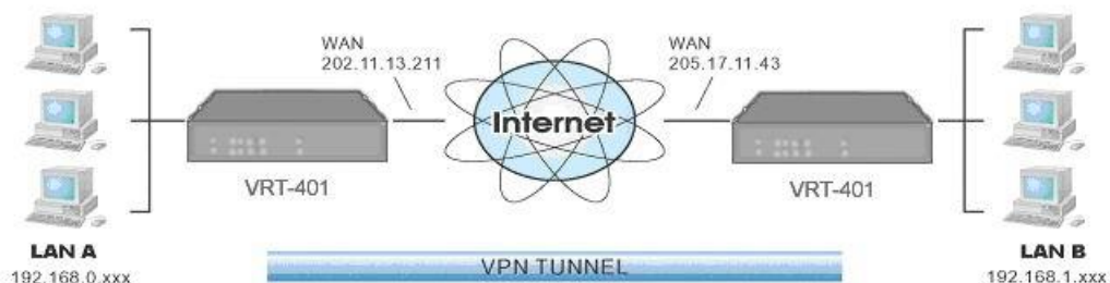
Figure 53: Connecting 2 VRT-401s
