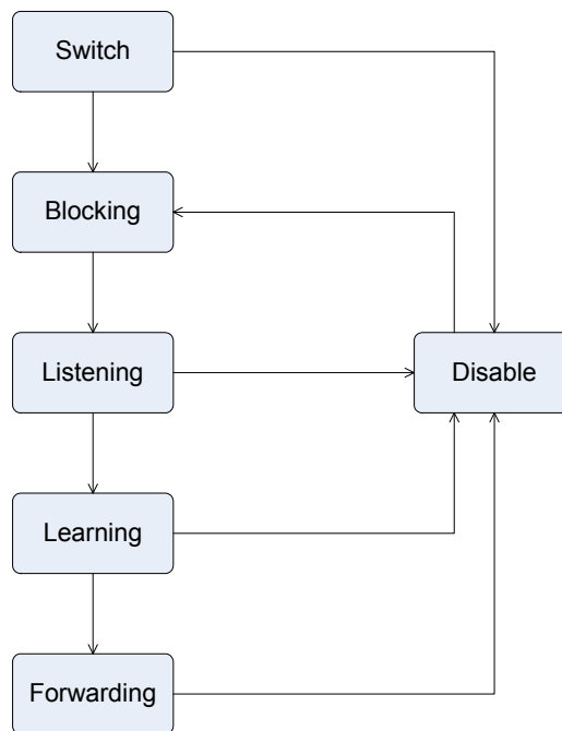
Figure 4-5-1: STP Port State Transitions
