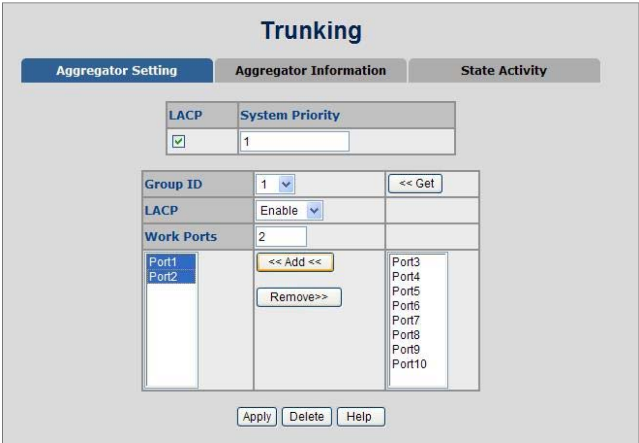
Figure 4-6-5: Switch 2 configuration interface
