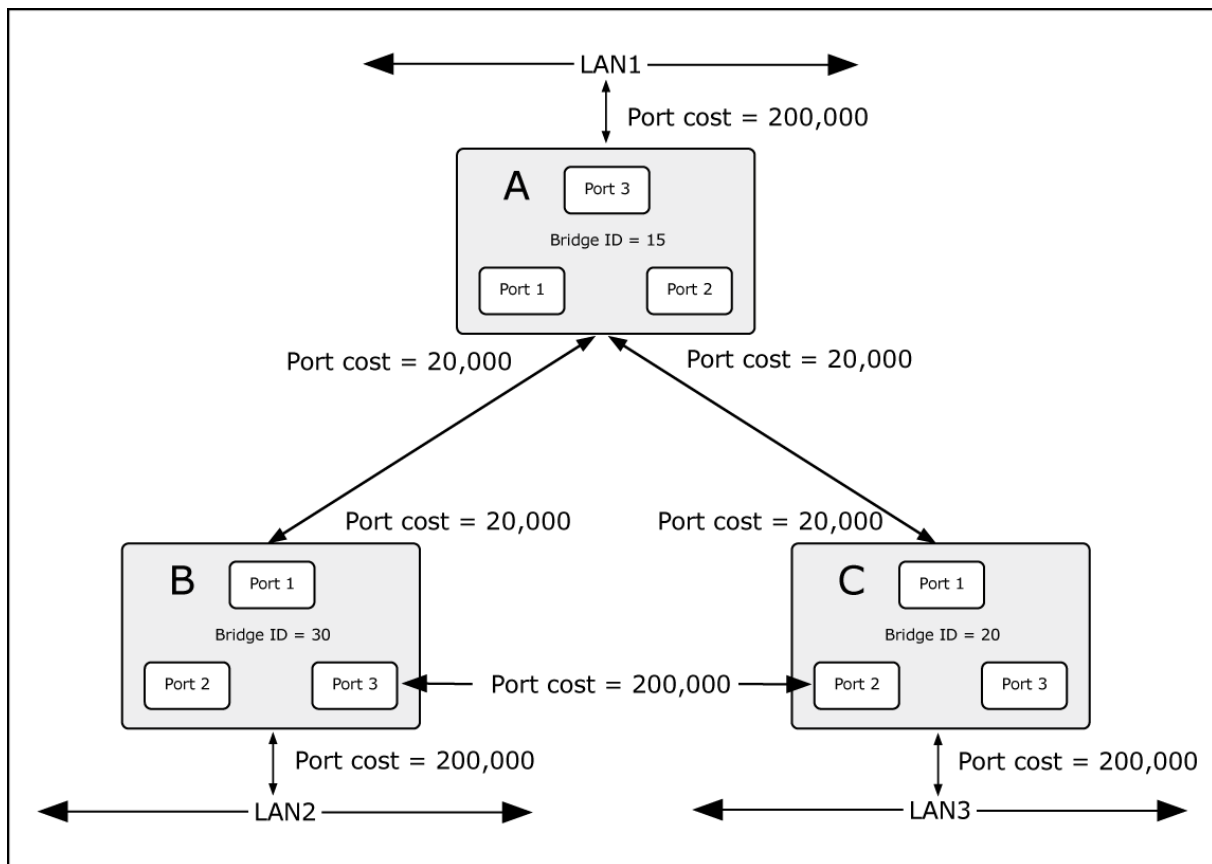
Figure 4-5-2: Before Applying the STA Rules
