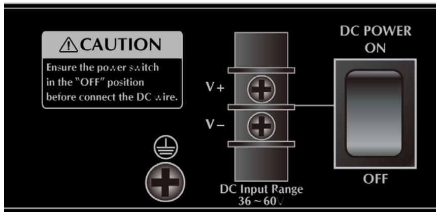
Figure 2-1-7 Rear Panel of GS-5220-16S8CR
