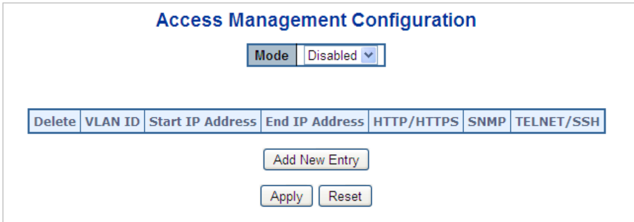
Figure 4-12-2: Access Management Configuration Overview Page Screenshot
