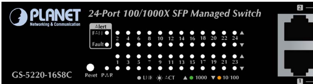
Figure 2-1-3: GS-5220-16S8C LED at Front Panel
