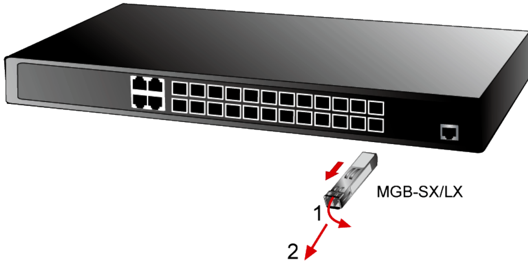
Figure 2-2-5: How to Pull Out the SFP Transceiver
