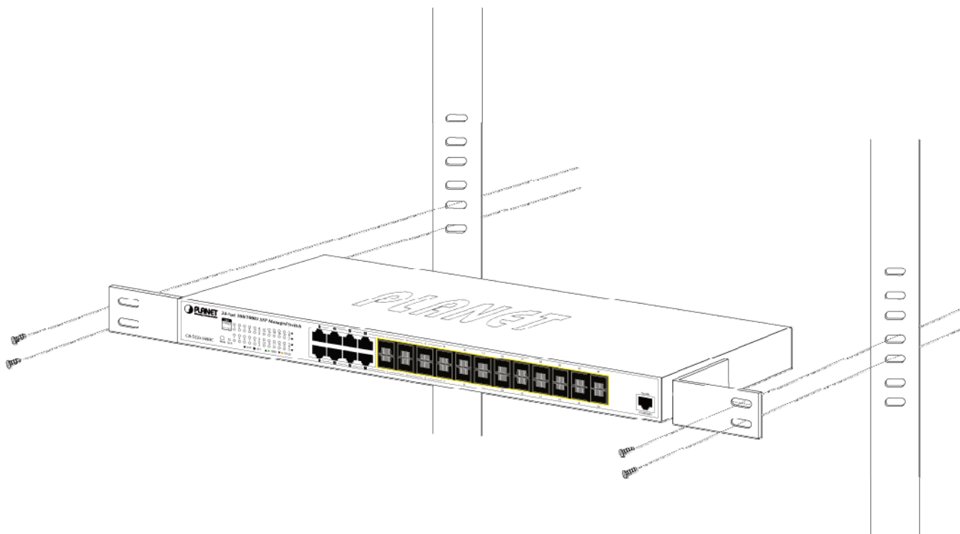
Figure 2-2-3: Mounting Managed Switch in a Rack
