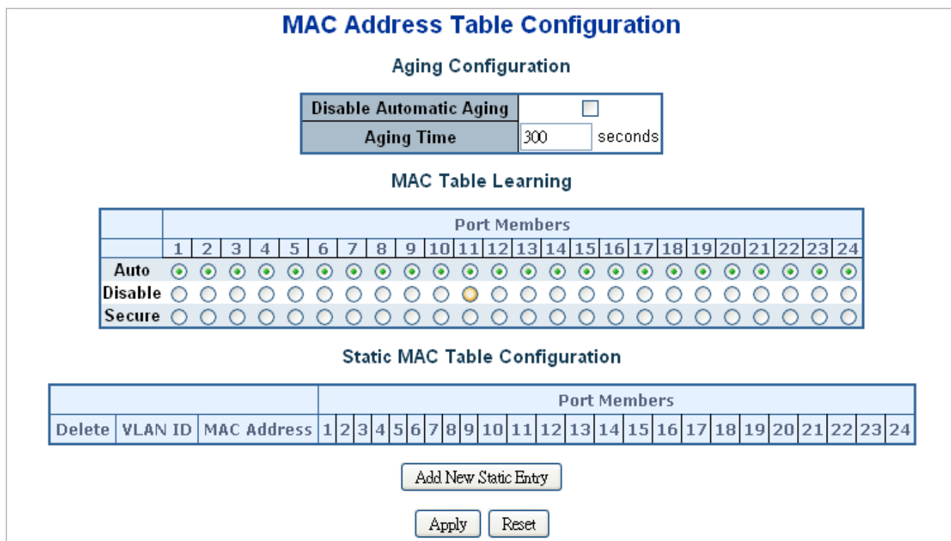
Figure 4-13-1: MAC Address Table Configuration Page Screenshot
