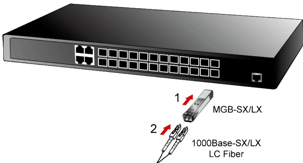
Figure 2-2-4: Plug-in the SFP Transceiver
