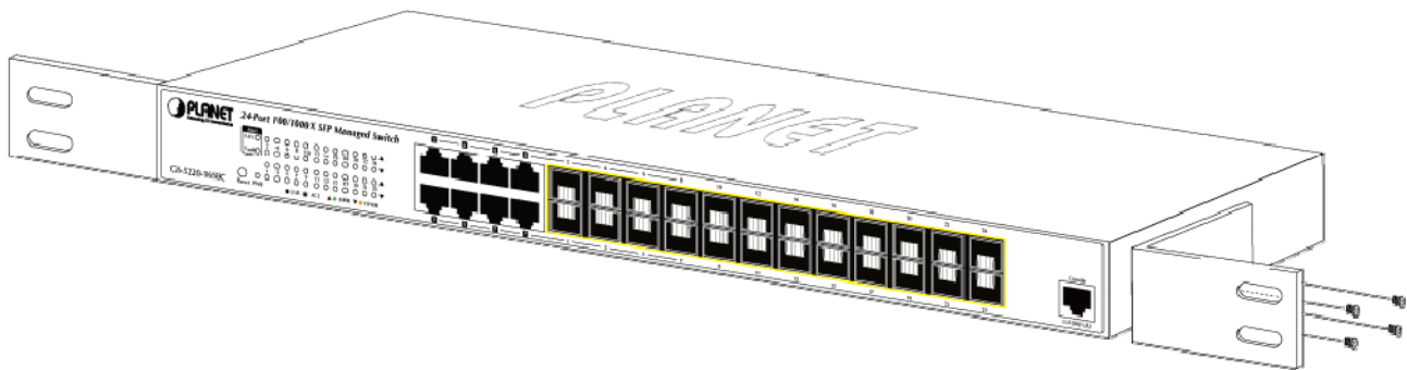
Figure 2-2-2: Attach Brackets to the Managed Switch.
