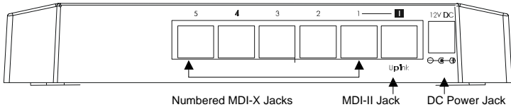
Rear panel of SW-500 and SW-800
