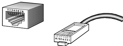
The standard cable, RJ-45 pin assignment
