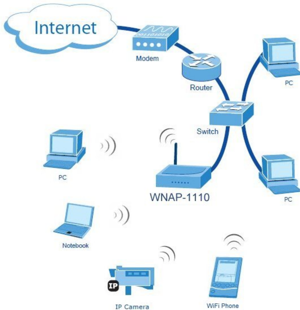
Figure 2-1 The Example of Infrastructure Network Incorporating the WNAP-1110
