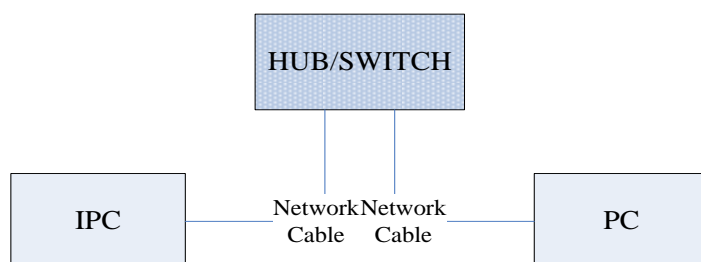
Figure 1 Network architecture
