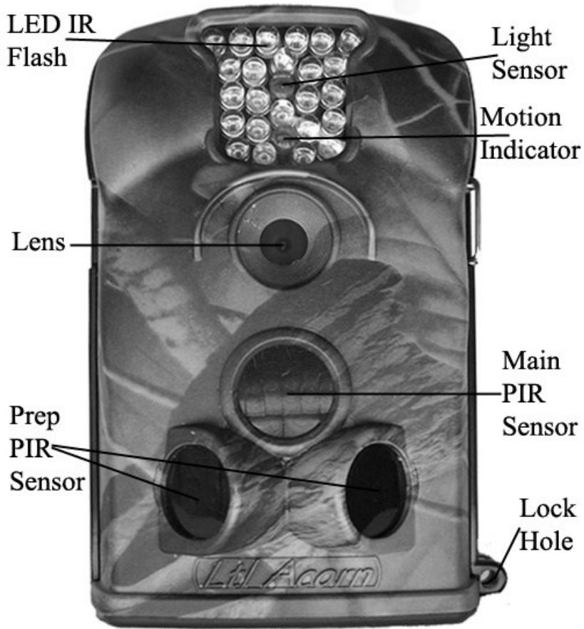
Figure 1.1: Front View
