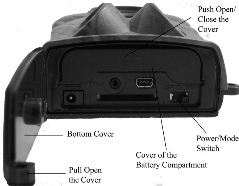
Figure 1.2: Bottom View
