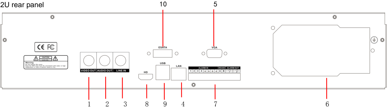
2U rear panel
